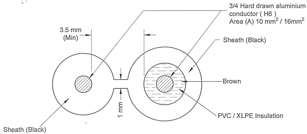
( a ) TWIN SERVICE MAIN WIRE ( PHASE CORE INSULATED, NEUTRAL CORE BARE & BOTH SHEATHED )
